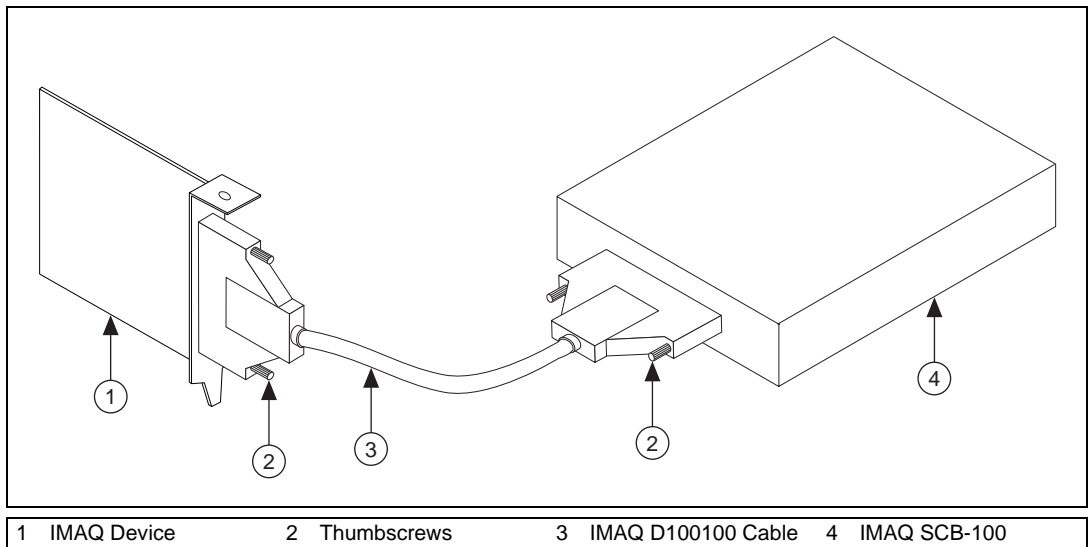
Figure 2. Connecting the D100100 Cable to Your IMAQ Device and IMAQ SCB-100
